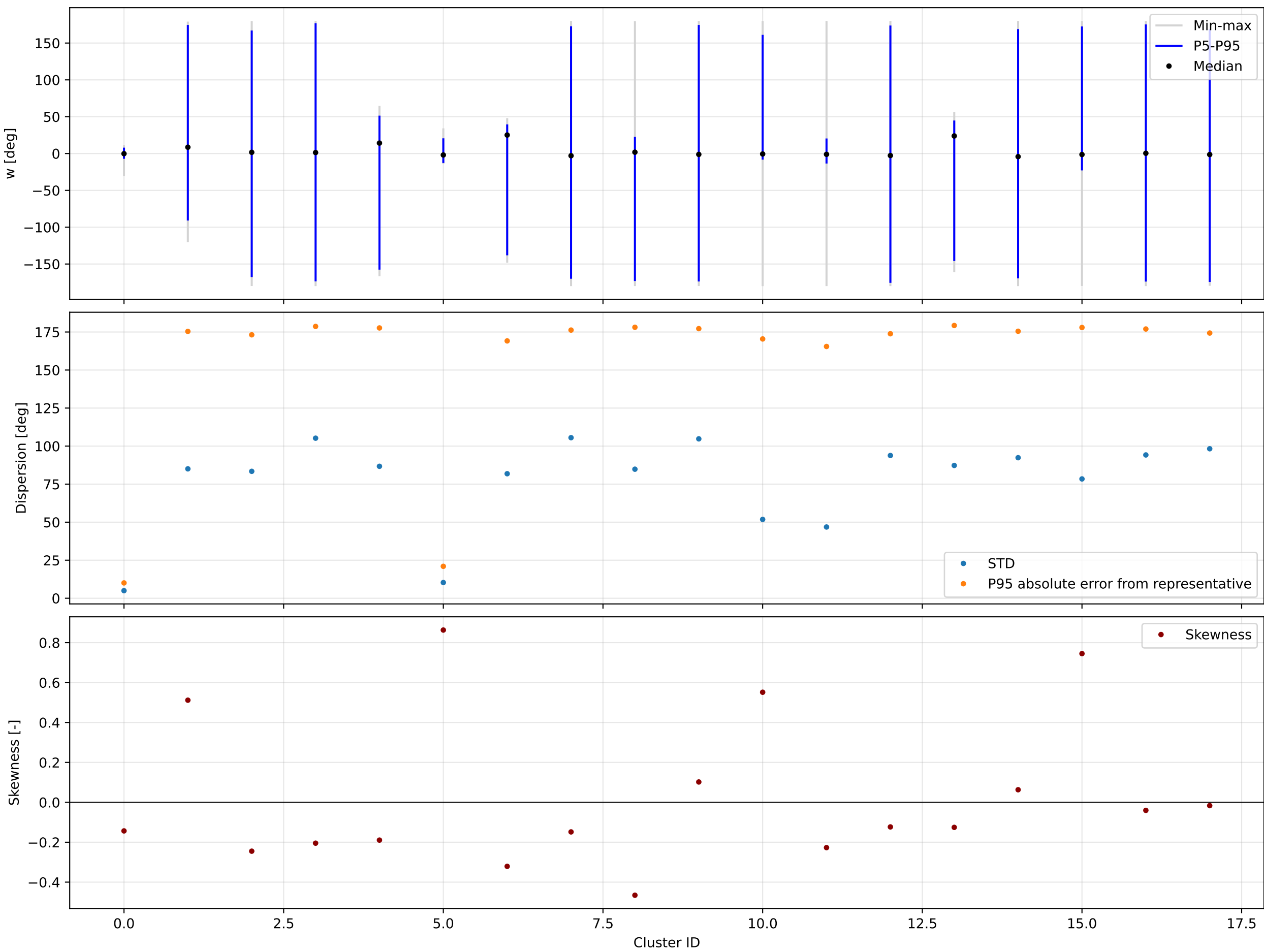
K=18 | forward | w | valid=194058/194058 | offsets from each cluster circular mean
