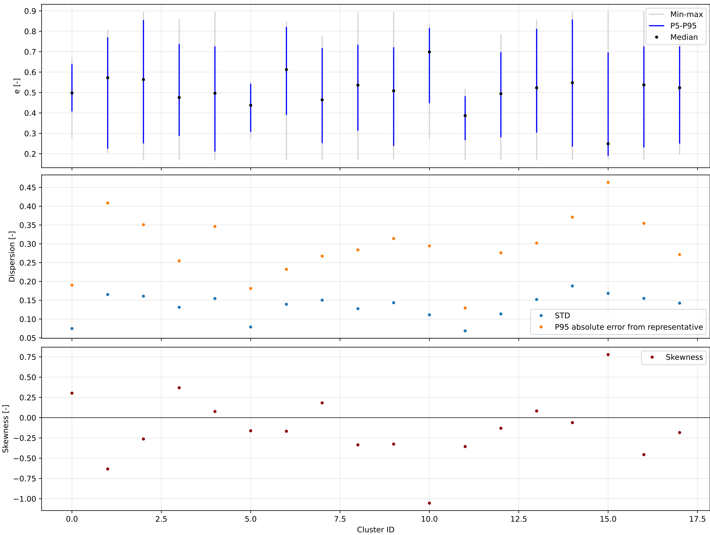
K=18 | backward | e | valid=194058/194058
