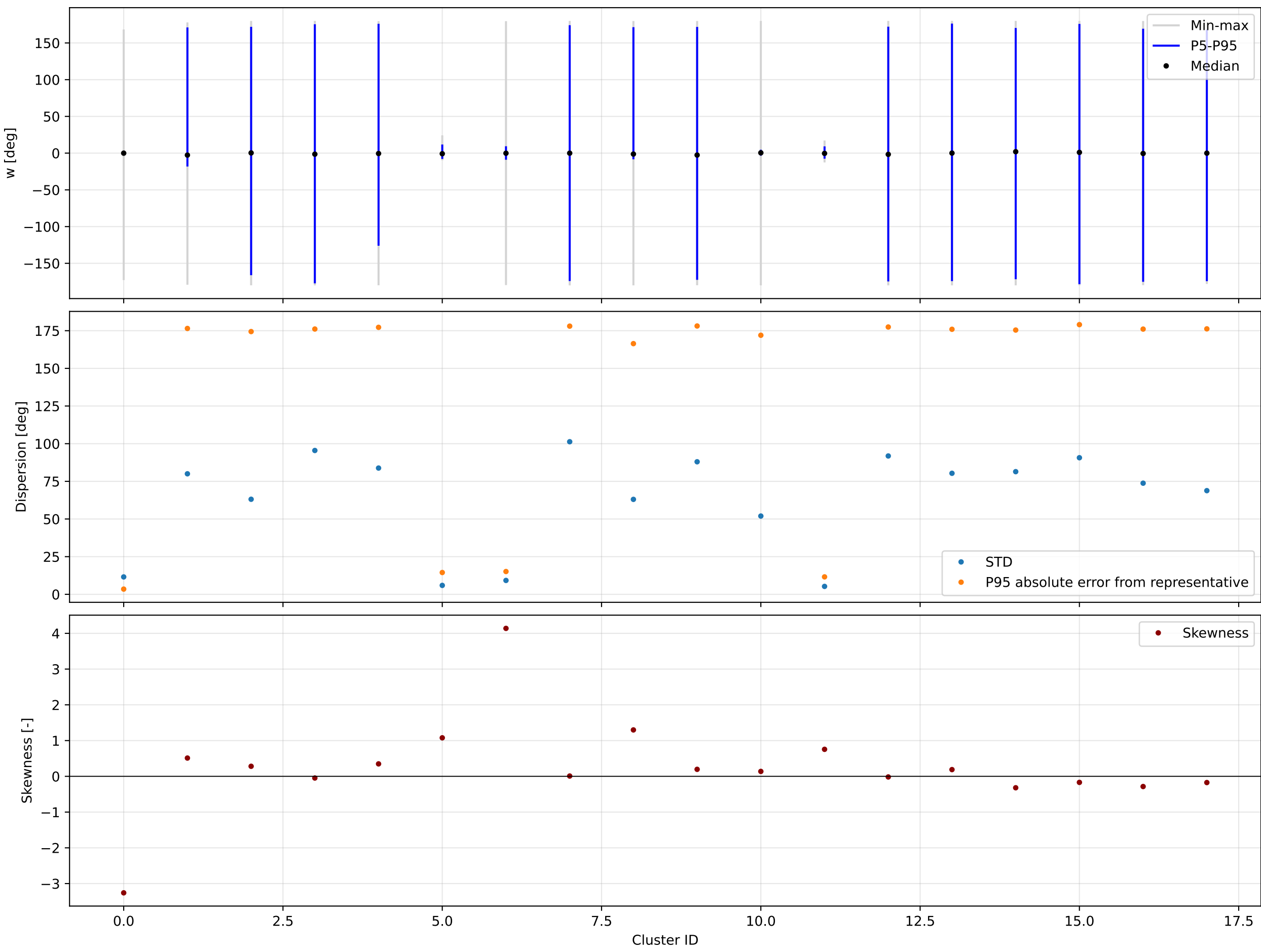
K=18 | backward | w | valid=194058/194058 | offsets from each cluster circular mean
