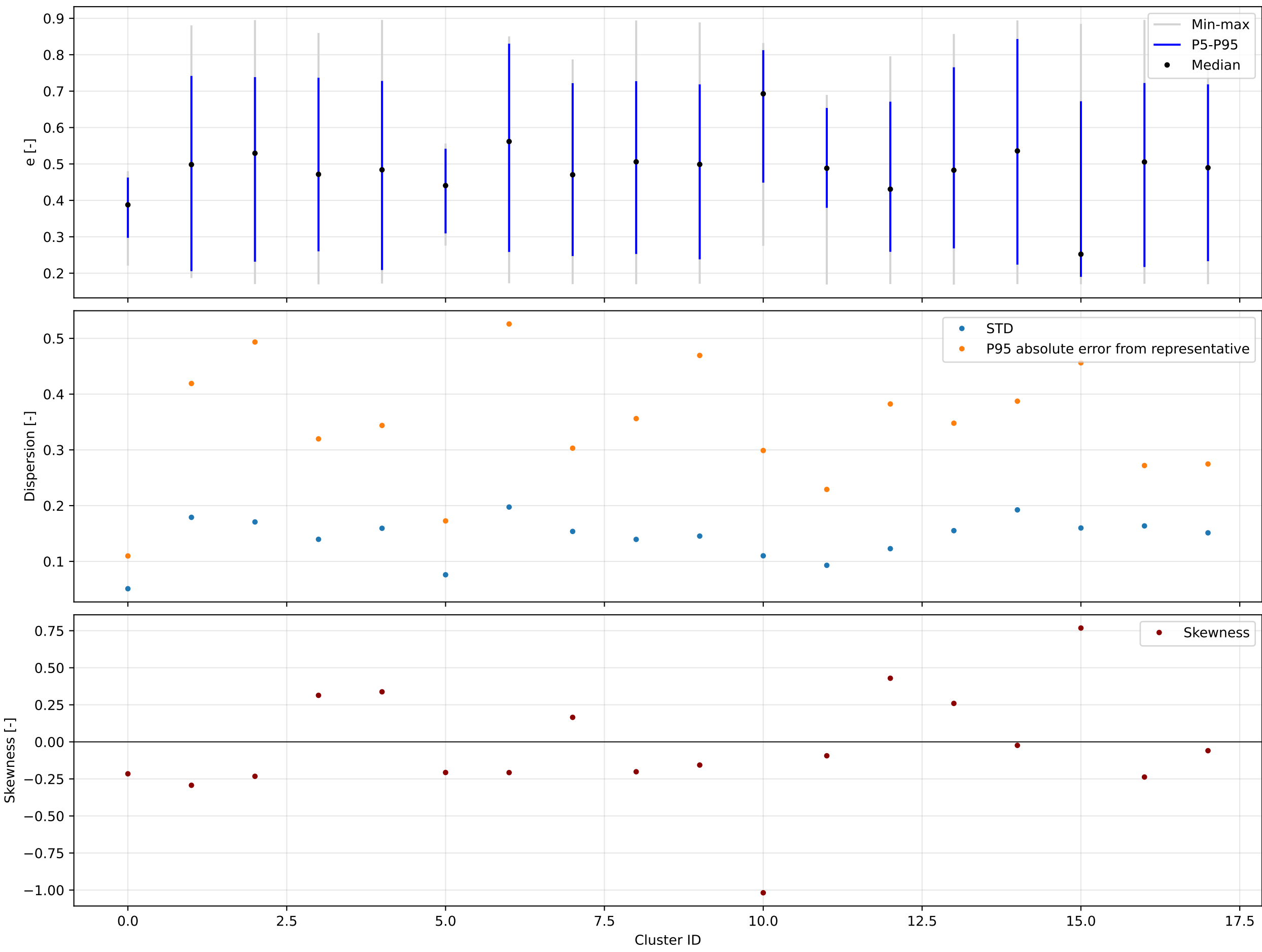
K=18 | forward | e | valid=194058/194058
